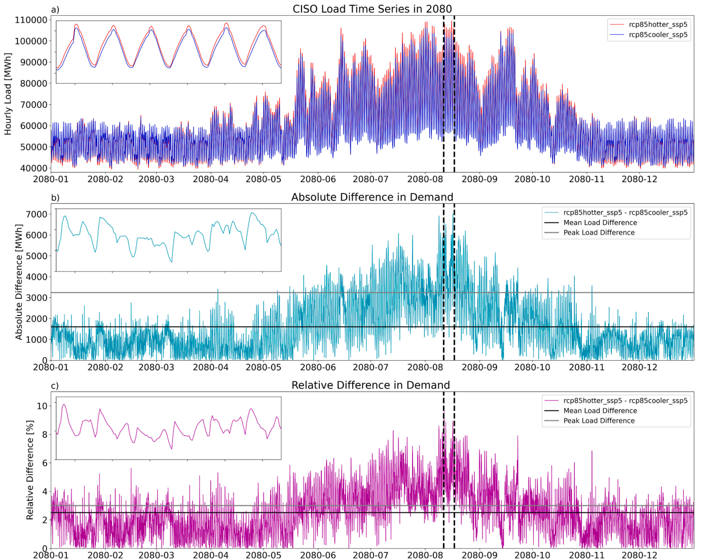
Fig. 2. Example of the calculation of mean and peak demand differences between the rcp85hotter_ssp5 and rcp85cooler_ssp5 scenarios for one year of TELL output in CISO: a) the 8760-h time series from the pair of scenarios; b) the hourly absolute demand difference between the pair; and c) the hourly relative demand difference between the pair. The inset in each panel shows the values zoomed in for a one-week period (vertical dashed lines) during a heat wave. The y-axis limits on the insets are the same as the plot they are embedded in.
