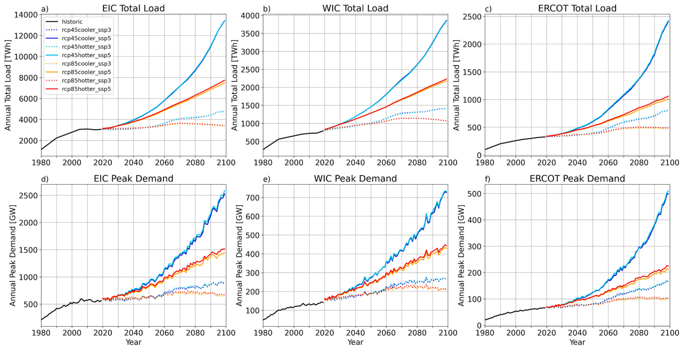
Fig. 3. Historical and projected annual total load (top row) and annual peak demand (bottom row) from 1980 to 2100. Projections using the SSP3 socioeconomic forcing are shown in the dashed lines while projections using the SSP5 forcing are solid lines. Climate scenarios are indicated by different color lines. The projections are shown for the three U.S. grid interconnections: the Eastern Interconnection (EIC; left column), Western Interconnection (WIC; center column), and Electricity Reliability Council of Texas (ERCOT; right column).
