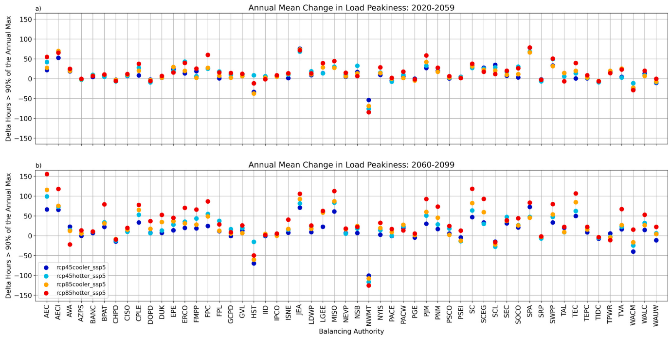
Fig. 9. Changes in the number of hours with loads that exceed 90 % of the annual maximum load (y-axes) by BA (x-axes). The top row shows the mean change by BA from 2020 to 2059 (i.e., the first repeat of the 40-year historical variability) and the bottom row shows the mean change from 2060 to 2099 (i.e., the second repeat). The different colors represent the four climate scenarios used in this analysis.
