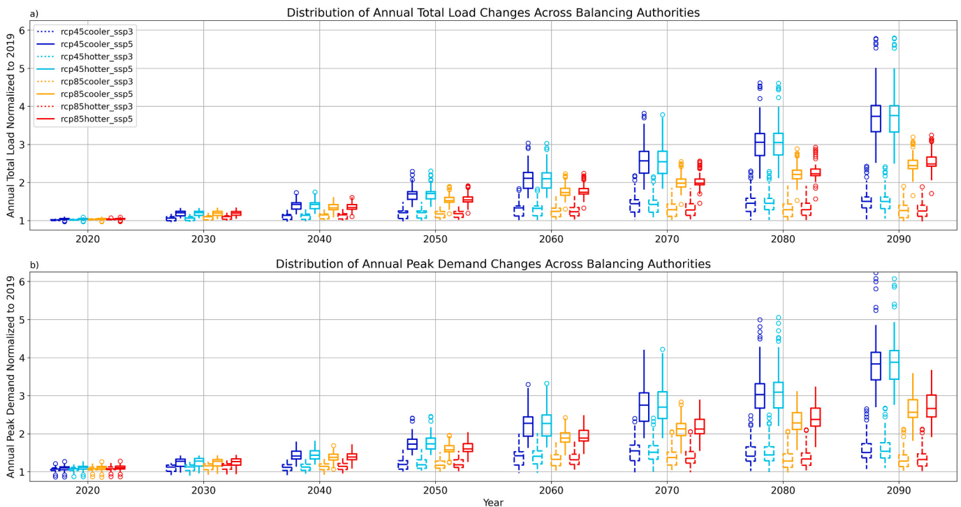
Fig. 4. Distribution across BAs of the change in annual total load (top row) and annual peak demand (bottom row) from 2020 to 2090 for each of the eight scenarios. Data is shown in 10-year increments to reduce clutter. Values are normalized to the 2019 historical loads to facilitate comparison across BAs and over time.
